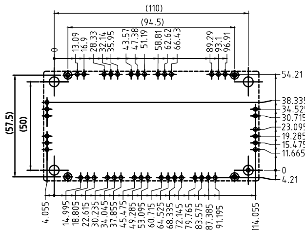
PCB hole pattern
