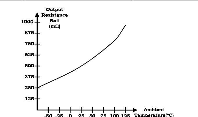
Fig. 10 On-state Status Output Resistance Versus Ambient Temperature
