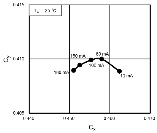
Fig. 8.4 Chromaticity - I_F
