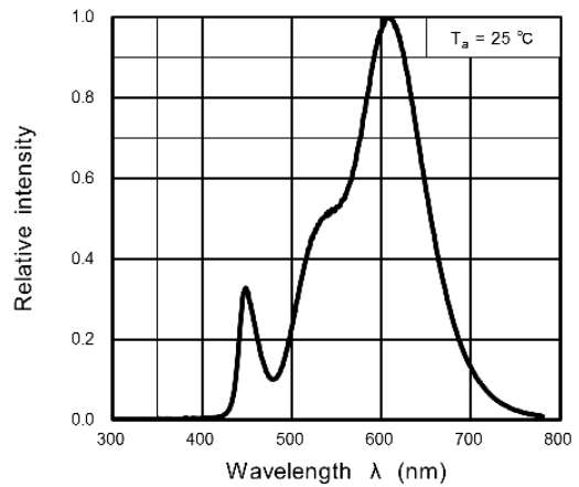
Fig. 8.6 Wavelength Characteristic
