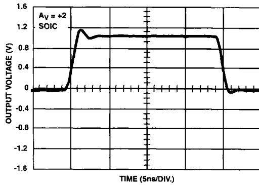
FIGURE 5. LARGE SIGNAL PULSE RESPONSE
