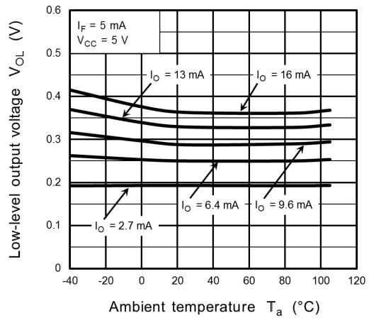
Fig. 12.2.6 V_{OL} - T_a
