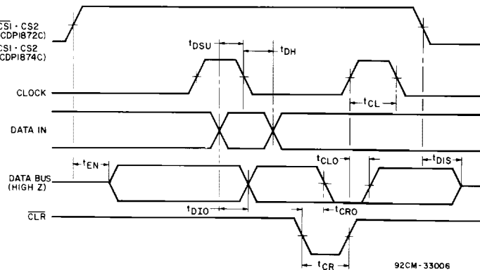
Fig. 4 - Timing waveforms for CDP1872C and CDP1874C (input-port types).
