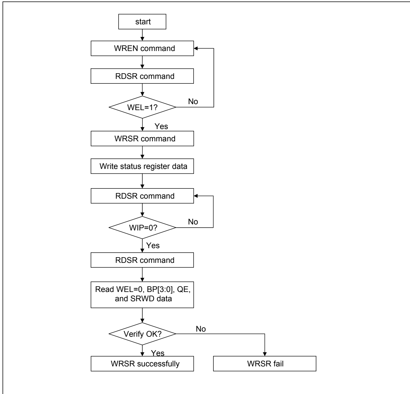
Figure 7. WRSR flow
