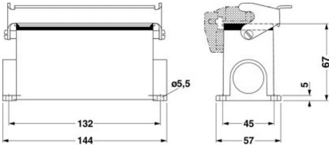
Dimensioned drawing
