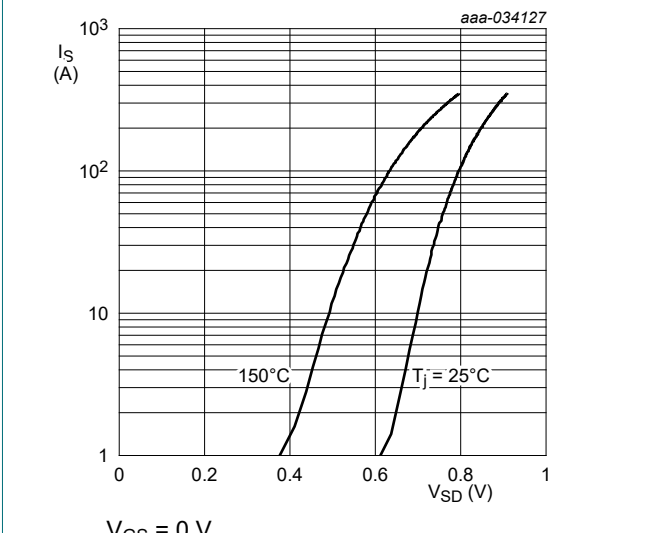
Fig. 15. Source-drain (diode forward) current as a function of source-drain (diode forward) voltage; typical values V_{GS} = 0 \text{ V}
