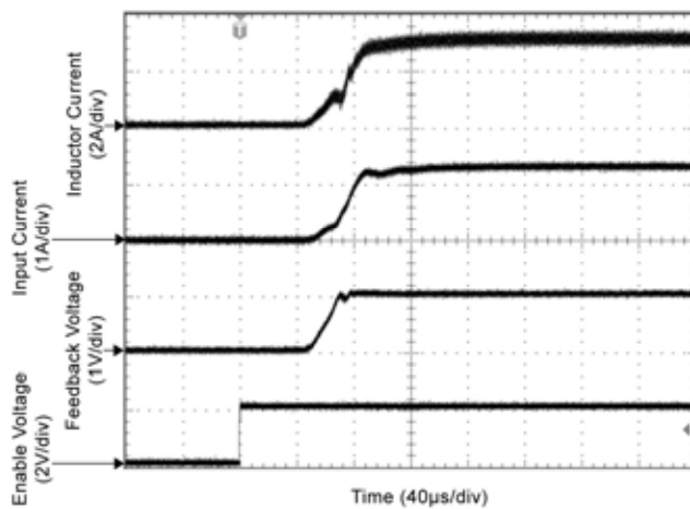
Start-Up Waveforms
