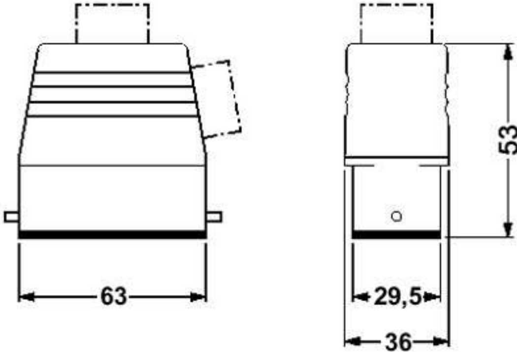
Dimensioned drawing
