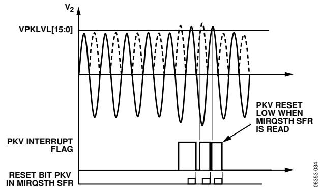
Figure 58. Peak Level Detection
