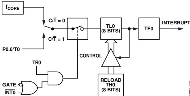
Figure 99. Timer/Counter 0, Mode 2
