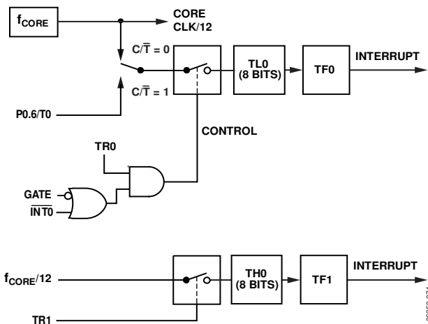
Figure 100. Timer/Counter 0, Mode 3
