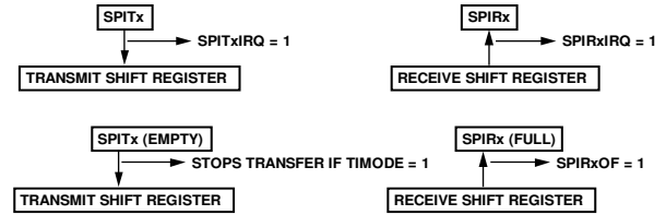
Figure 111. SPI Receive and Transmit Interrupt and Status Flags
