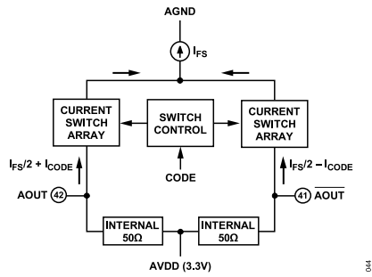
Figure 27. DAC Output
