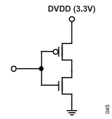
Figure 29. CMOS Input
