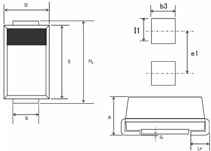
DO-214AC(SMA), (FVDS)
