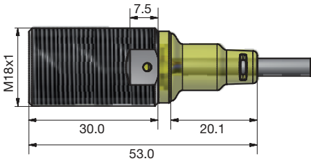
Fig. 22 Short body, flush version, cable
