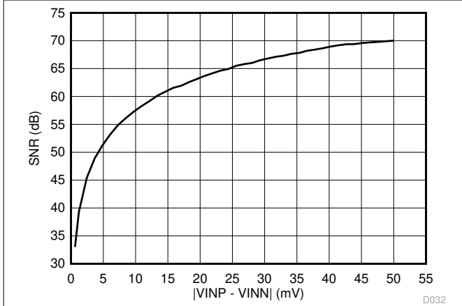
Figure 6-25. Signal-to-Noise Ratio vs Input Voltage
