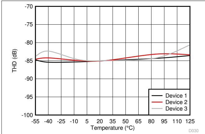
Figure 6-23. Total Harmonic Distortion vs Temperature
