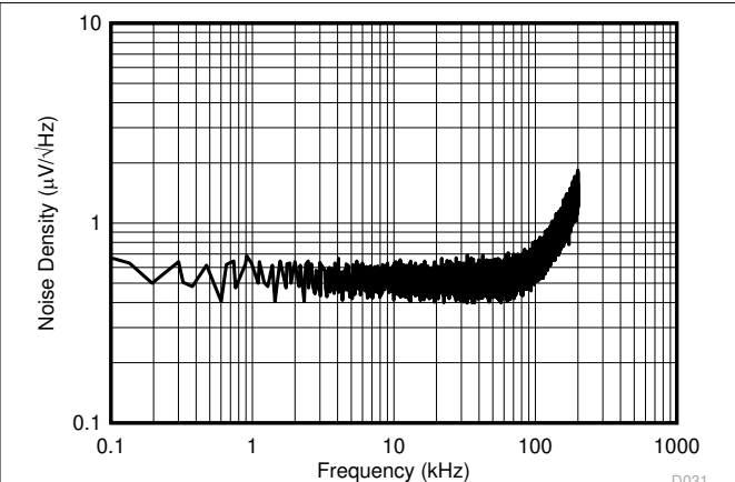
Figure 6-24. Output Noise Density vs Frequency
