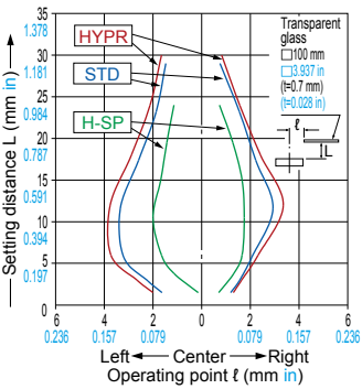
FD-L31A Reflective type
