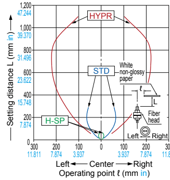
FD-S21 Reflective type
