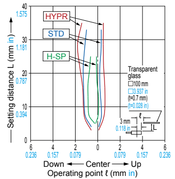
FD-L31A Reflective type
