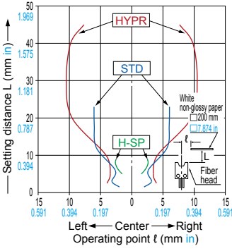
FD-L21W Reflective type
