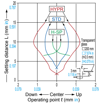
FD-L23 Reflective type
