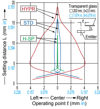
FD-L22A Reflective type
