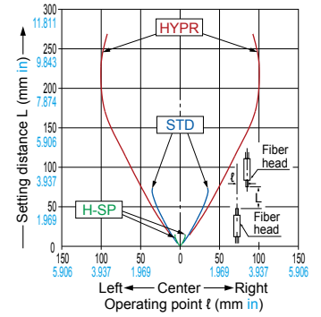
FT-E23 Thru-beam type
