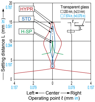
FD-L23 Reflective type
