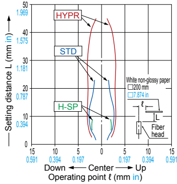
FD-L21W Reflective type
