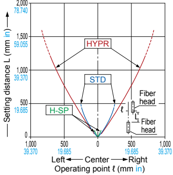
FT-H35-M2 Thru-beam type FT-H35-M2S6
