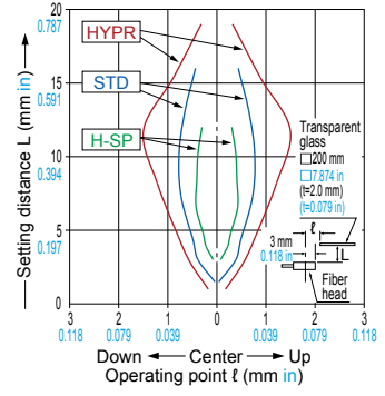
FD-L22A Reflective type
