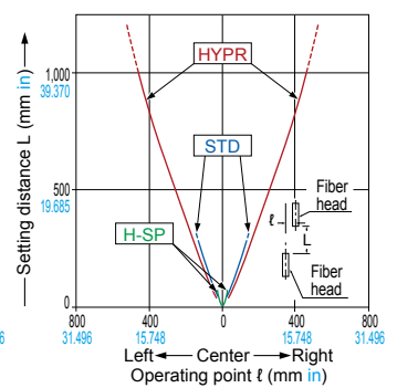
FT-H30-M1V-S Thru-beam type
