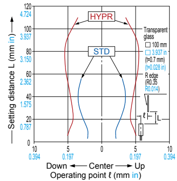
FD-L32H Reflective type
