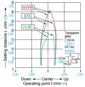
FD-L30A Reflective type
