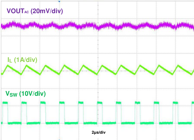
Figure 24. Output Ripple V_{IN}=12\text{V} , V_{OUT}=5\text{V} , I_{OUT}=50\text{mA} , PWM
