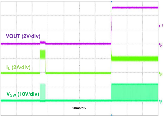
Figure 36. Output Short Recovery, I_{OOUT} = 2\text{A}
