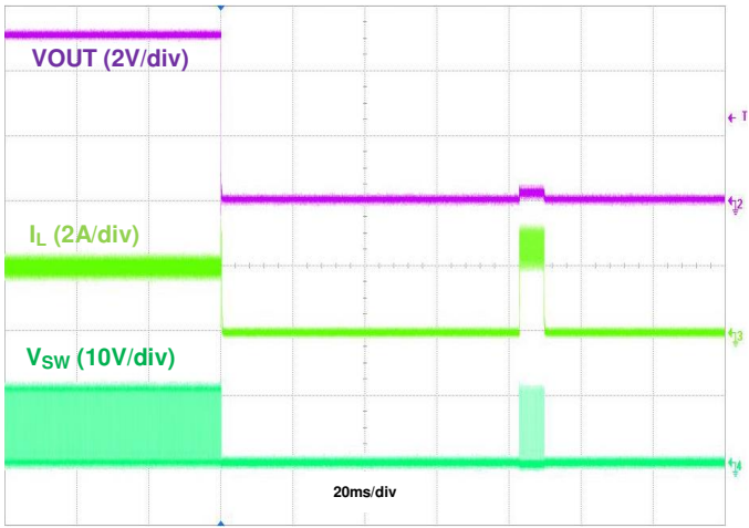
Figure 35. Output Short Protection, I_{OOUT} = 2\text{A}
