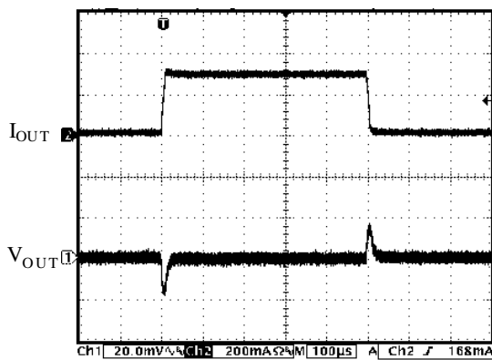
Load Transient (Conditions: C IN =C OUT =1μF, V IN =4.4V, V OUT =3.3V)
