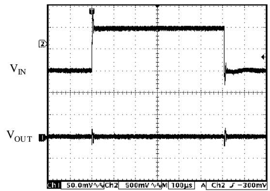
Line Transient (Conditions: I OUT =30mA, C IN =C OUT =1μF, V IN =2.5 to 3.5V, V OUT =0.8V)
