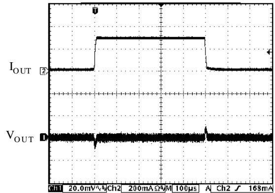
Load Transient (Conditions: C IN =C OUT =1μF, V IN =2.5V, V OUT =0.8V)
