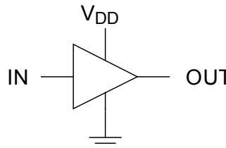
Figure 51. Non-Inverting Driver
