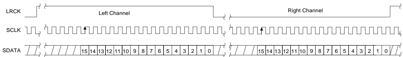
Figure 24. CS43L41 Format 4
