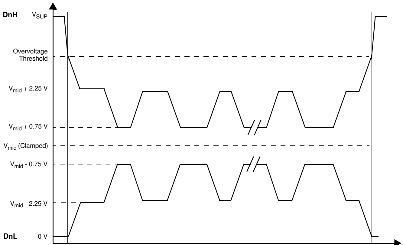
Figure 6. DBUS Overtolerance Bus Waveforms
