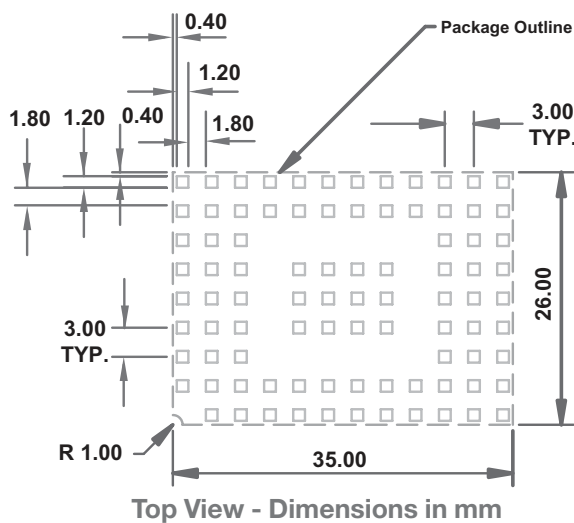
Figure 8 Footprint Dimensions
