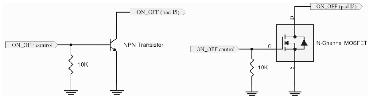
Figure 5 ON / OFF Driver
