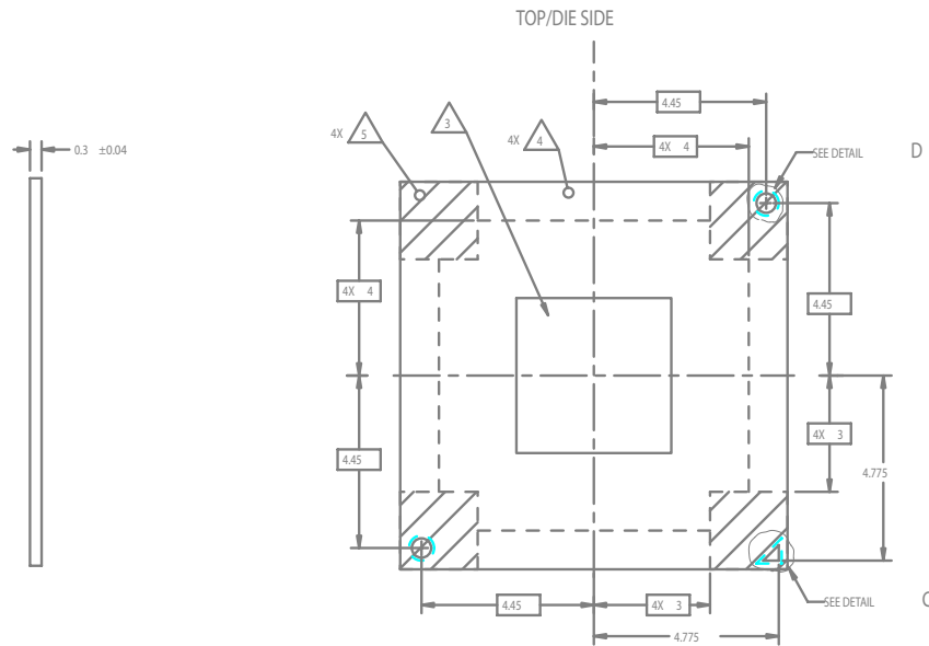
Figure 6. Mechanical Drawing (2 of 4)
