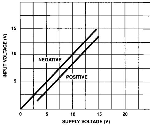
FIGURE 1. INPUT VOLTAGE RANGE vs SUPPLY VOLTAGE
