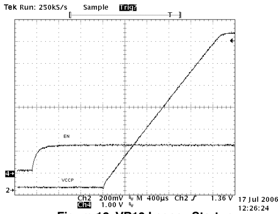
Figure 16. VR10 Legacy Startup
