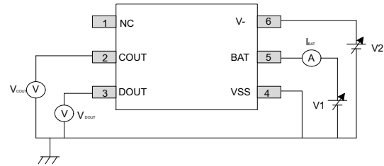
Figure 8-4. Test Circuit 2
