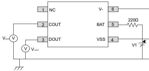
Figure 8-3. Test Circuit 1
