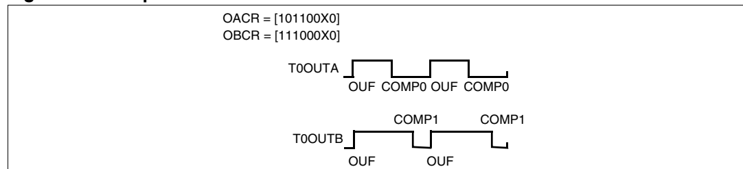
Figure 114. Output waveforms
