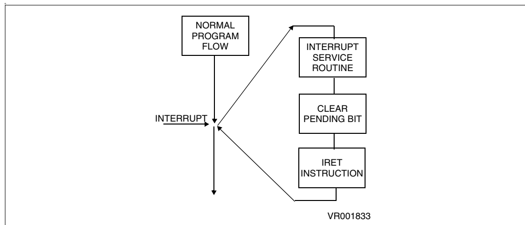
Figure 44. Interrupt response
