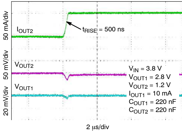
Figure 44. Load Transient Response – Rising Edge, I_{OUT} = 50 \text{ mA} to 150 \text{ mA}
