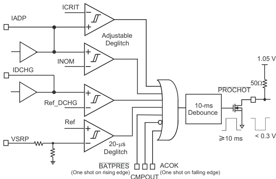
Figure 6. PROCHOT Profile
