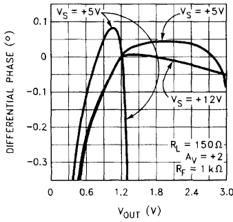
Differential Phase for Single Supply Operation
