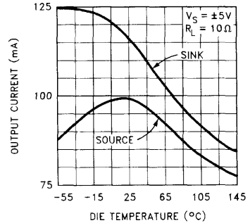
Output Current vs Die Temperature
