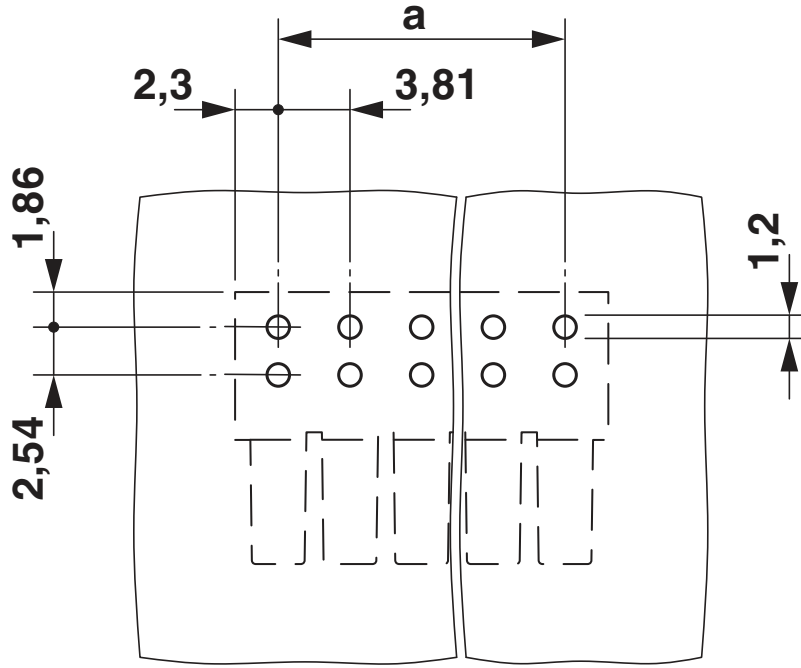
Drilling diagram
