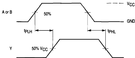
Figure 1. Switching Waveforms
