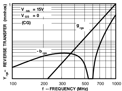
Reverse Transadmittance
