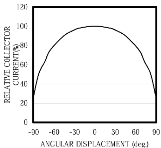
ANGULAR DISPLACEMENT
