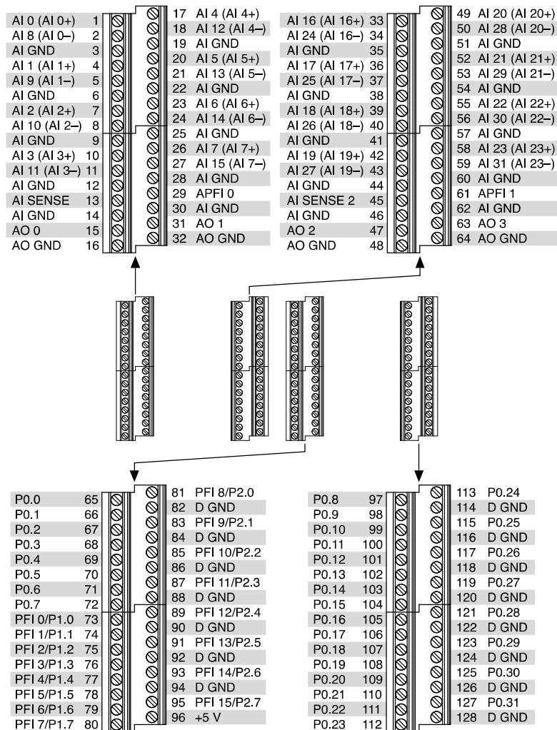
Figure 11. NI USB-6289 Screw Terminal Pinout
