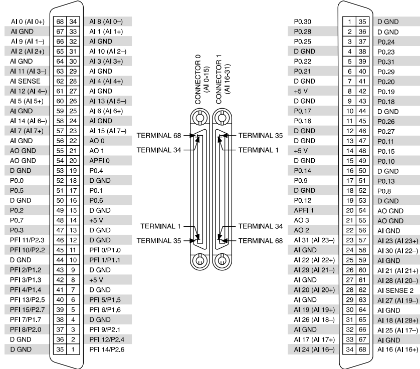
Figure 9. NI PCI/PXI-6289 Pinout
