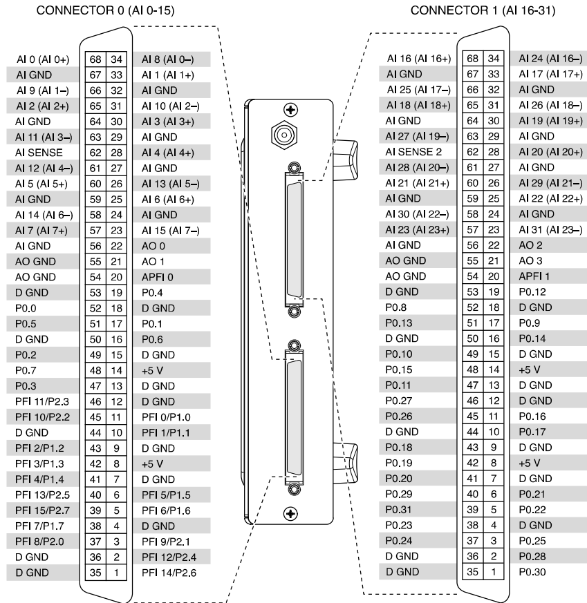
Figure 10. NI USB-6289 Mass Termination Pinout
