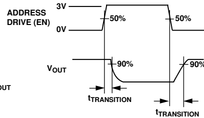
Figure 21. Switching Time of Multiplexer, t_{\text{TRANSITION}}
