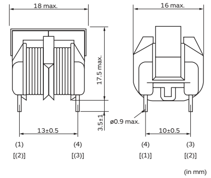
Standard Winding
