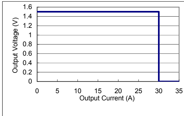
Fig. 7 Typical over-current of AGQ100-48S1V5
