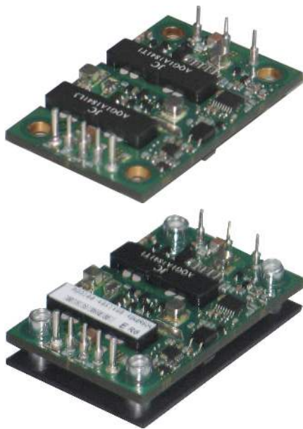
Industry Standard Quarter Brick : 2.28"X 1.45" X 0.38" (open frame) or 2.28" x 1.45" x 0.5" (baseplate)
