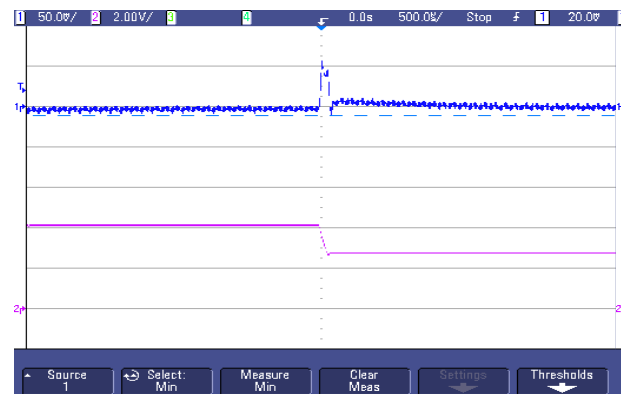
Fig.31 Typical transient response to step decrease in load from 50% to 25%, room temperature, 48Vdc input ( \Delta I_o/\Delta t = 0.1A/1\mu s ) of AGQ100-48S1V2
