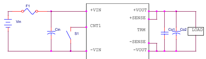
Fig. 60 Typical application
