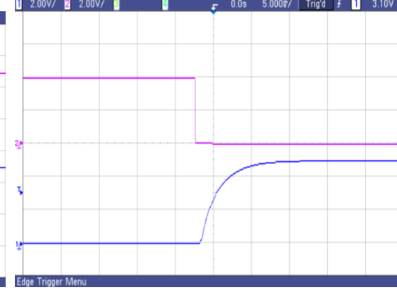
Fig.30 Typical start-up from CNT on of AVQ100B-48S05
