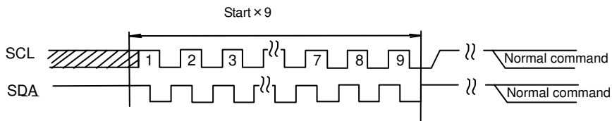
Figure 34.-(c) START×9 + command input
