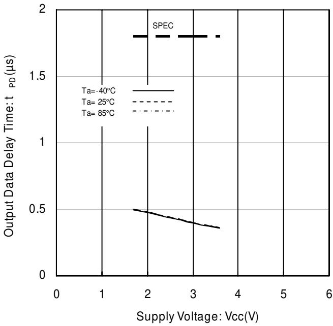
Figure 20. Output Data Delay Time vs Supply Voltage (LOW)
