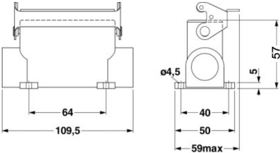
Dimensioned drawing
