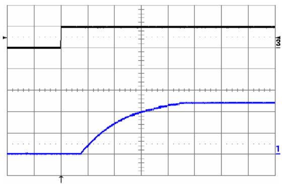
Figure 18. Turn-on transient at full rated load current (resistive) plus 2,200 \mu\text{F} at V_{in} = 48\text{ V} , triggered via ON/OFF pin. Top trace: ON/OFF signal (5 V/div.). Bottom trace: output voltage (5 V/div.). Time scale: 2 ms/div.
