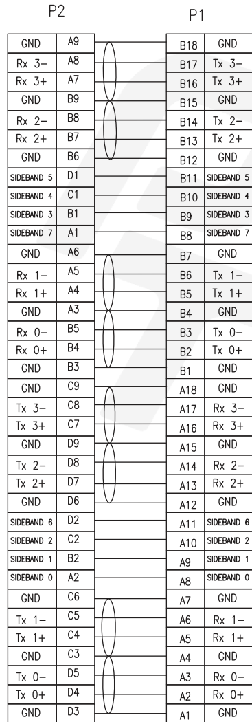
WIRING DIAGRAM
