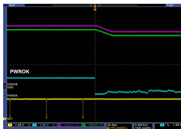
Figure 12: PWROK De-assertion
