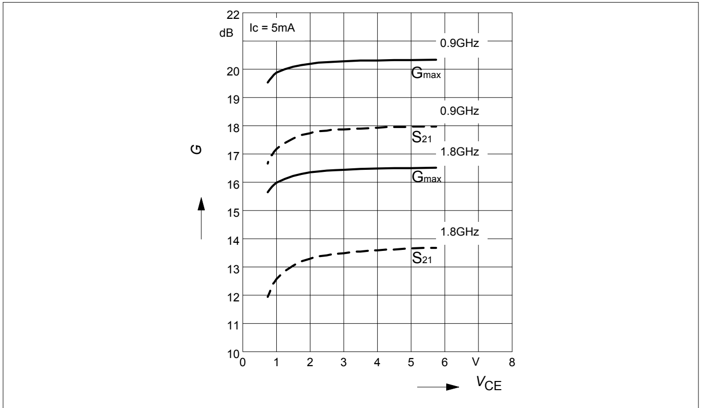
Figure 10 Maximum power gain G_{max} = f(V_{CE}) , transducer gain IS_{21}^2 = f(V_{CE}) , I_C = 5\text{ mA} , f = \text{parameter in GHz}
