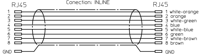
Wiring Diagramm Connection: INLINE
