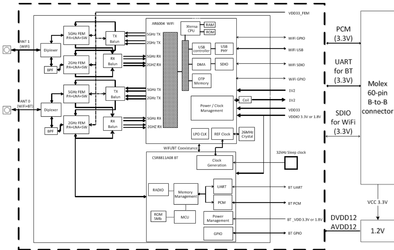
Figure 1: MSD50NBT block diagram
