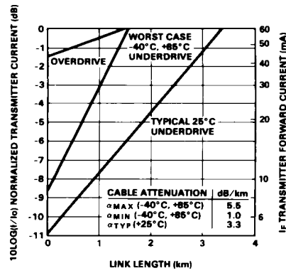
Figure 4. HFBR-14X2/ HFBR-24X2 link design limits with 100/ 140 µm cable.
