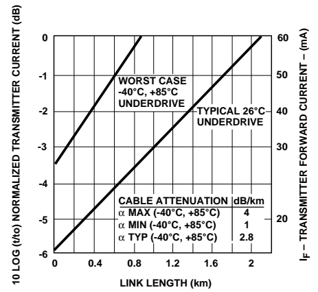
Figure 5. HFBR-14X4/ HFBR-24X2 link design limits with 50/ 125 µm cable.
