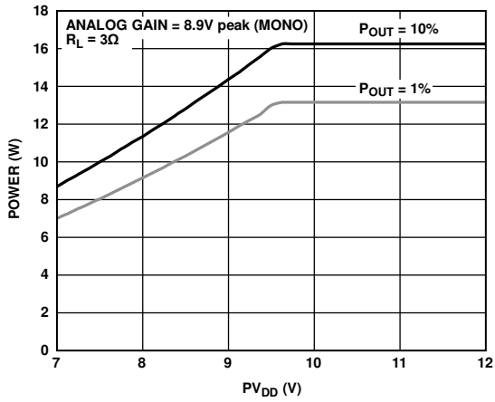
Figure 68. Power vs. PV DD , Analog Gain = 8.9 V peak, R L = 3 Ω
