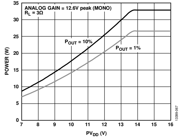
Figure 69. Power vs. PV DD , Analog Gain = 12.6 V peak, R L = 3 Ω
