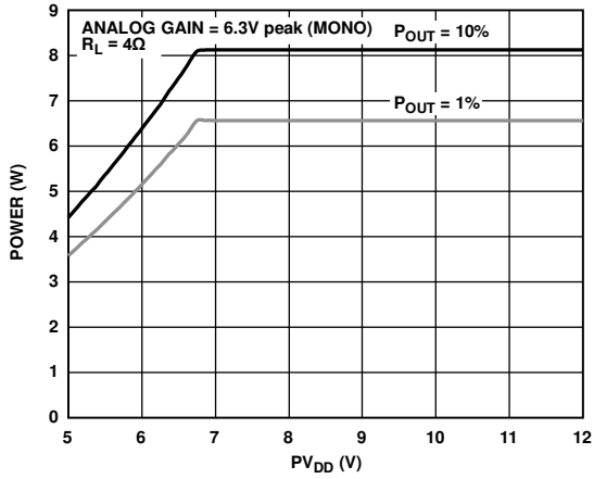
Figure 67. Power vs. PV DD , Analog Gain = 6.3 V peak, R L = 4 Ω
