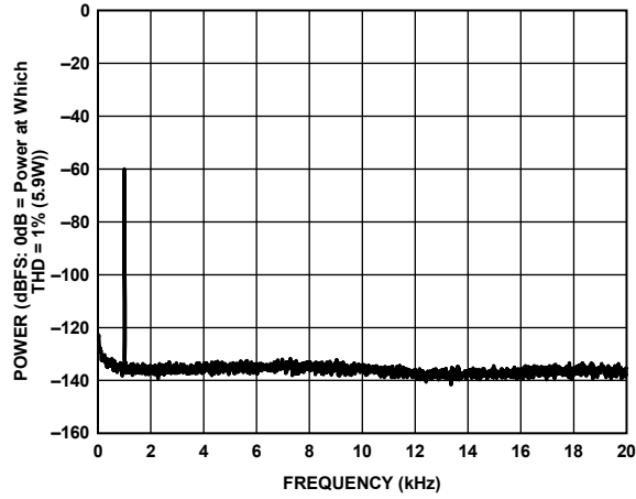
Figure 7. -60 dBFS Output Power into 4 Ω Load
