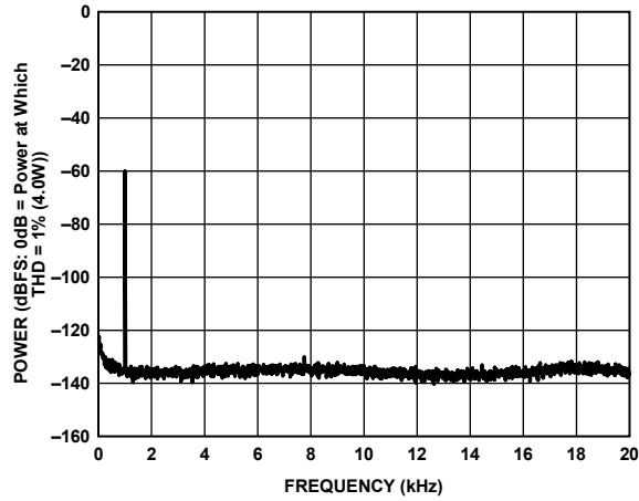
Figure 8. -60 dBFS Output Power into 6 Ω Load
