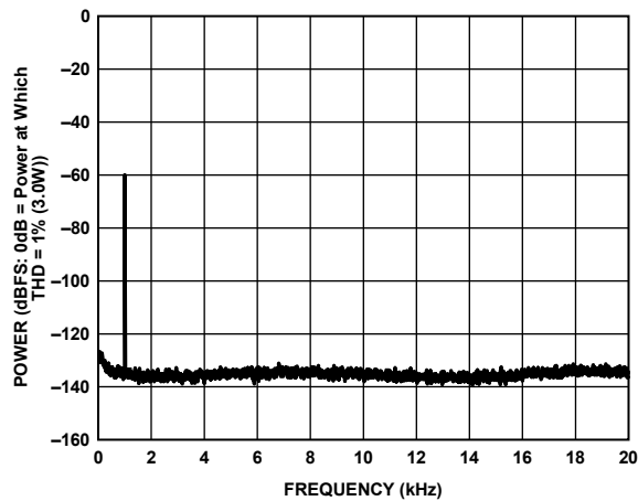
Figure 9. -60 dBFS Output Power into 8 Ω Load
